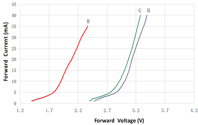
Forward Current VS. Forward Volt (Ta=25°C)
