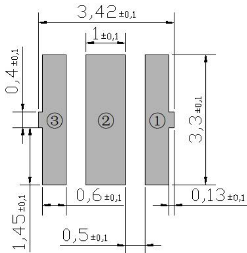
焊盘建议大小 Recommended size of pad
