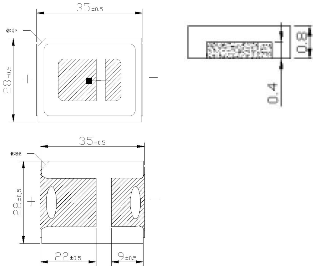
焊盘建议大小 Recommended size of pad
