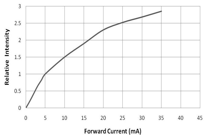
Relative Intensity VS. Forward Current (Ta=25℃)
