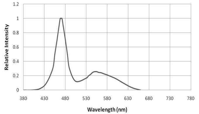
Spectrum Distribution (Ta=25℃)
