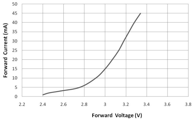
Forward Current VS. Forward Voltage (Ta=25℃)
