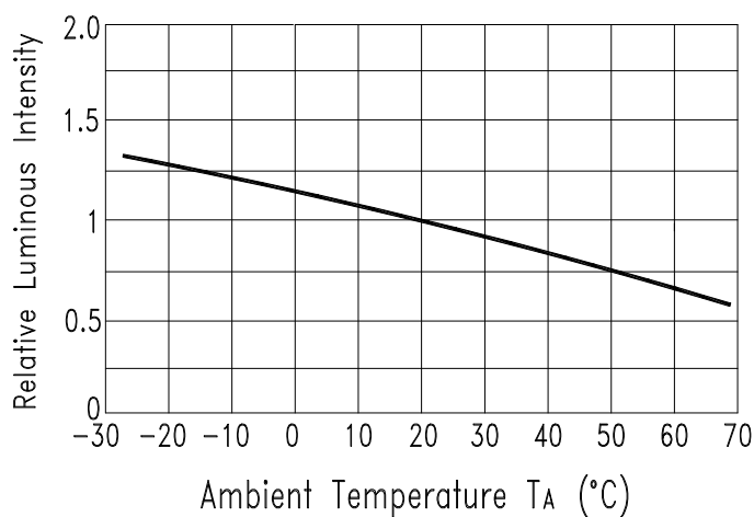
Fig.5 Luminous Intensity vs. Ambient Temperature
