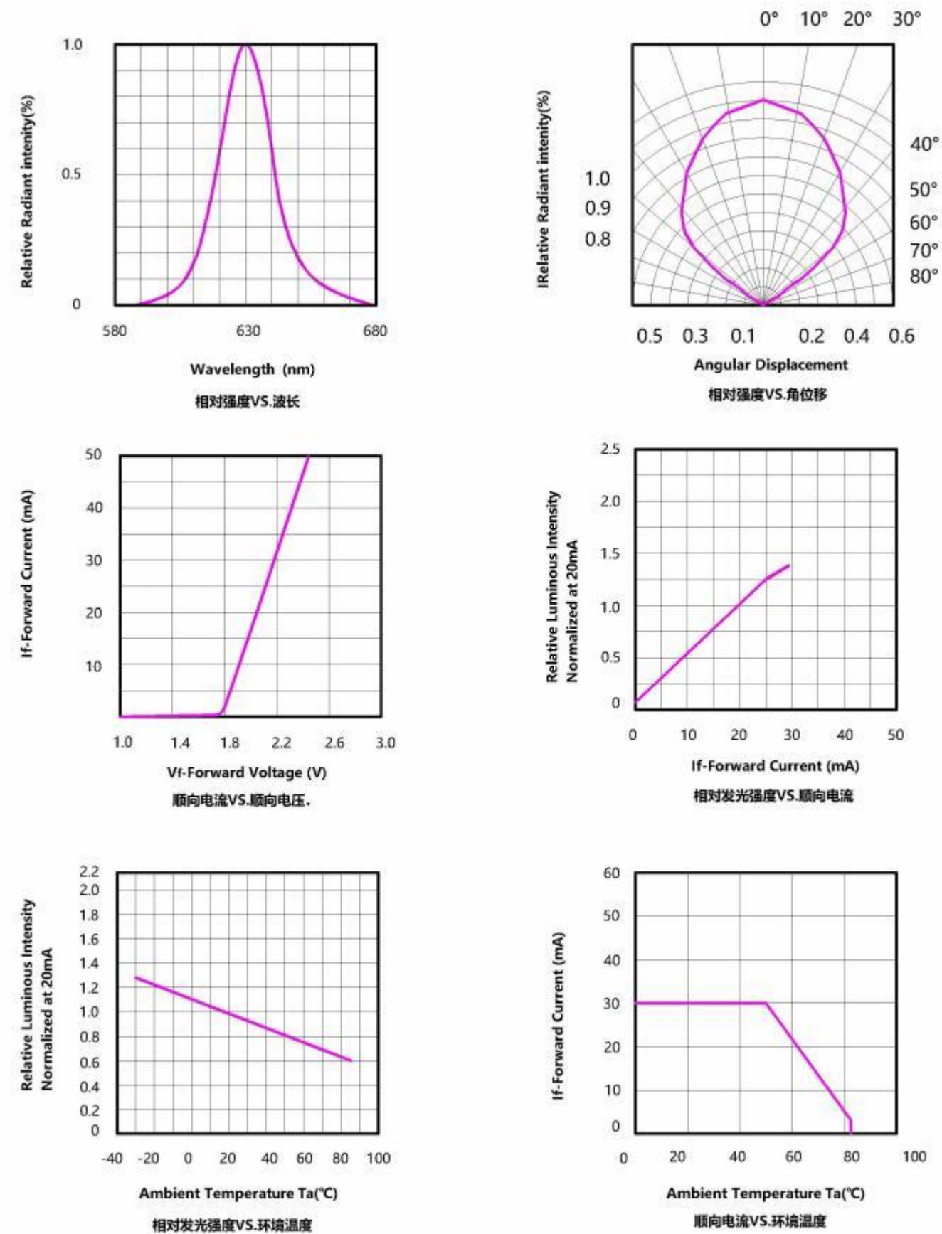
典型光电特性曲线图 Typical photoelectricity characteristic curve chart
