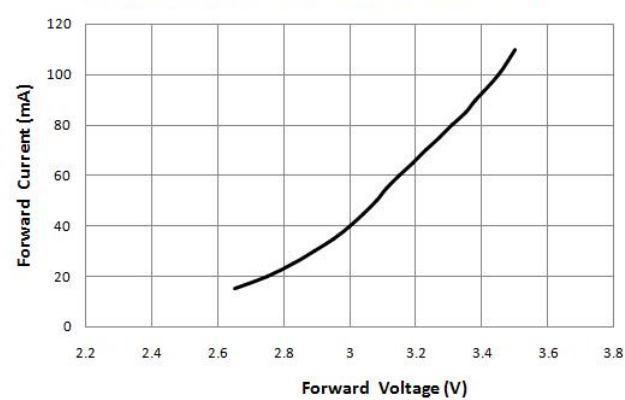
伏安特性曲线 Forward Current VS. Forward Voltag (Ta=25℃)
