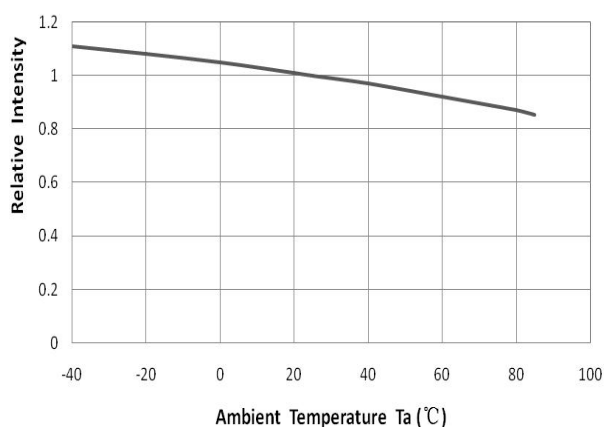
Relative Intensity VS. Ambient Temperature (Ta=25℃)
