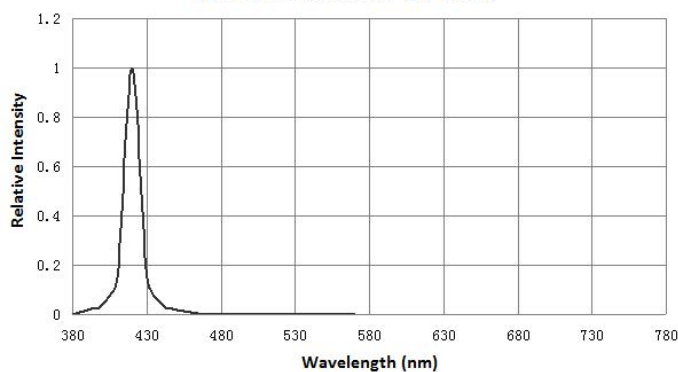
Spectrum Distribution (Ta=25℃)
