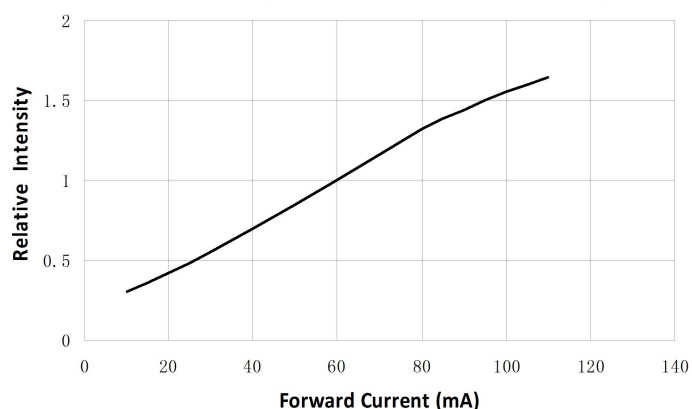
Relative Intensity VS. Forward Current (Ta=25℃)
