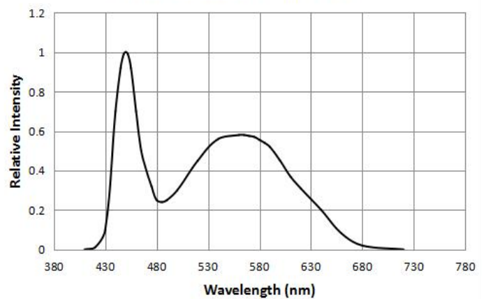
Spectrum Distribution (Ta=25°C)
