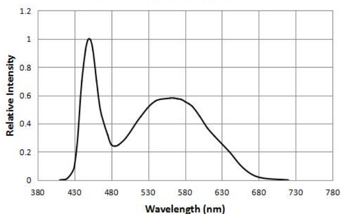
Spectrum Distribution (Ta=25℃)
