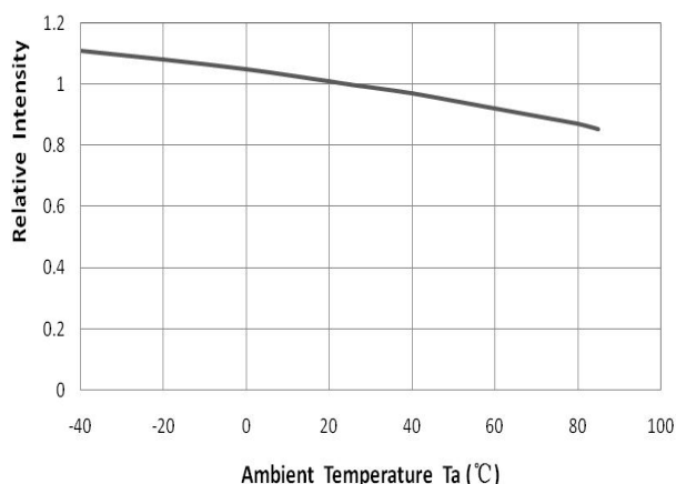
Relative Intensity VS. Ambient Temperature (Ta=25℃)
