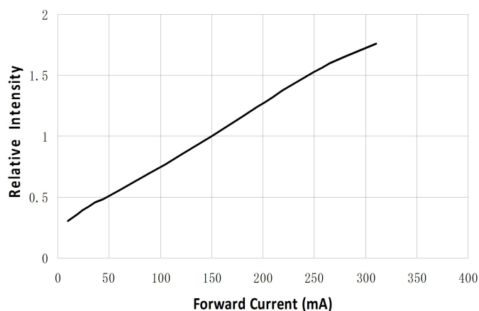
Relative Intensity VS. Forward Current (Ta=25℃)
