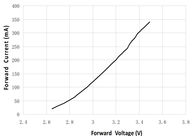
Forward Current VS. Forward Voltag (Ta=25℃)
